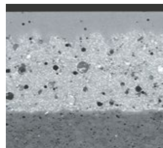
CEFIONTECT WC-Mikrograph * 1 µm=0,001 mm CEFIONTECT toilet micrograph * 1 µm=0.001 mm
