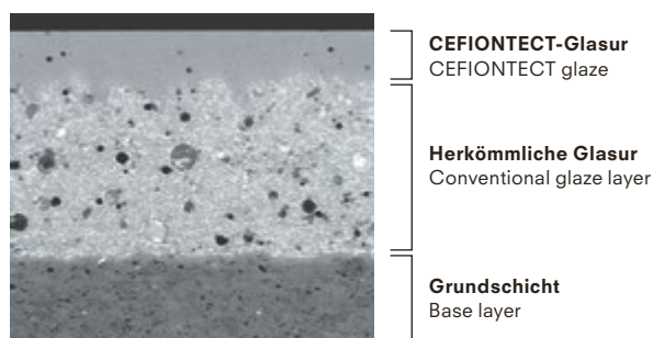
CEFIONTECT WC-Mikrograph * 1\ \mu\text{m}=0,001\ \text{mm} CEFIONTECT toilet micrograph * 1\ \mu\text{m}=0.001\ \text{mm}
